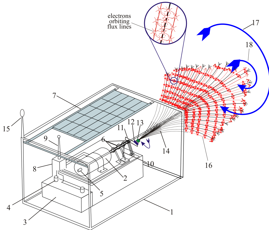
Fig.1. Machine to capture and energized charged particles (electrons and protons) by producing external magnetic field ( ExMF ).
