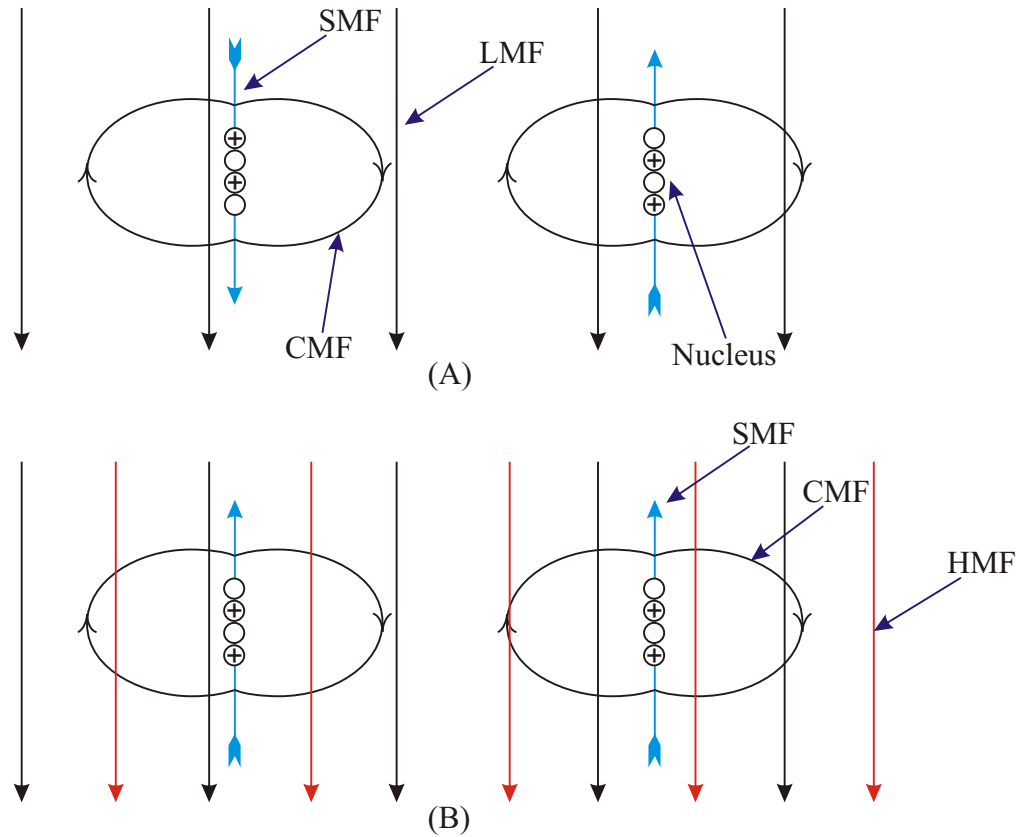
Fig.2. At micro scale, spinning magnetic field ( SMF ) [3] of helium; a diamagnetic element interacted with low magnetic field ( LMF ) in (A) no effect is caused in the nucleus. Increasing field intensity as in (B) helium's SMF re-arranged itself, thus opposing the imposed field.
