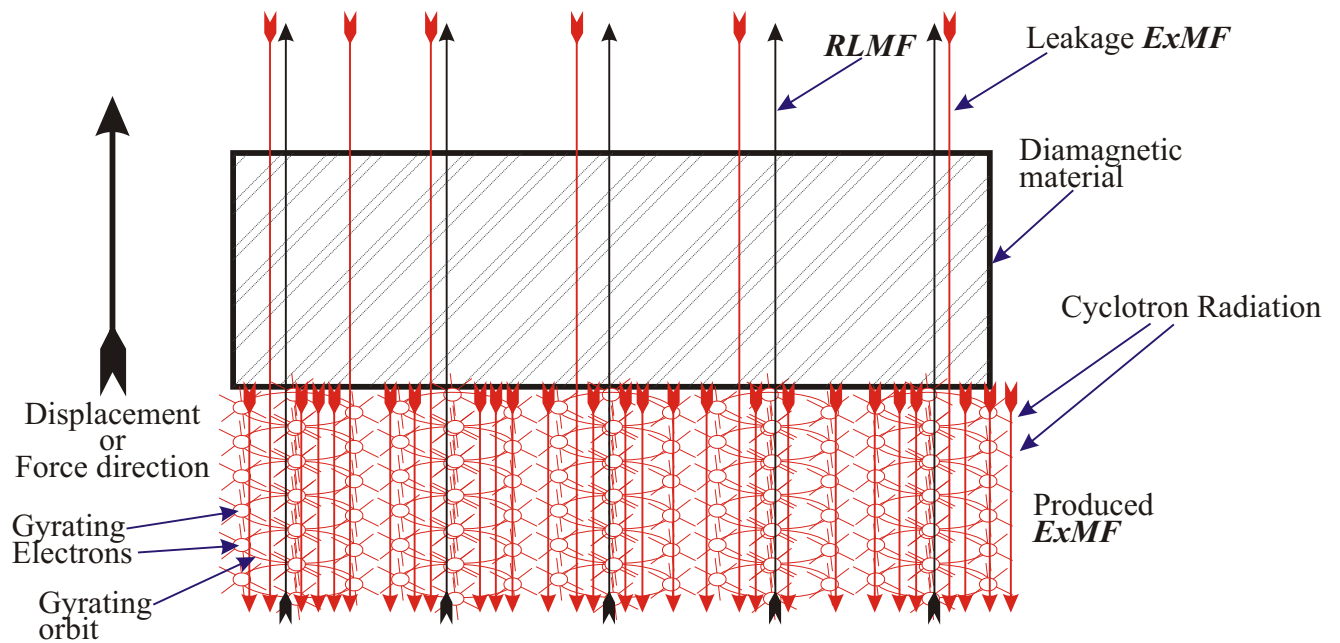
Fig.3. Rotating low magnetic field ( RLMF ) penetrating bismuth, interacted with electrons, producing external magnetic fields ( ExMF )[4]. The produced ExMF interacts with the bismuth producing a translational (displacement) force, with direction shown.
