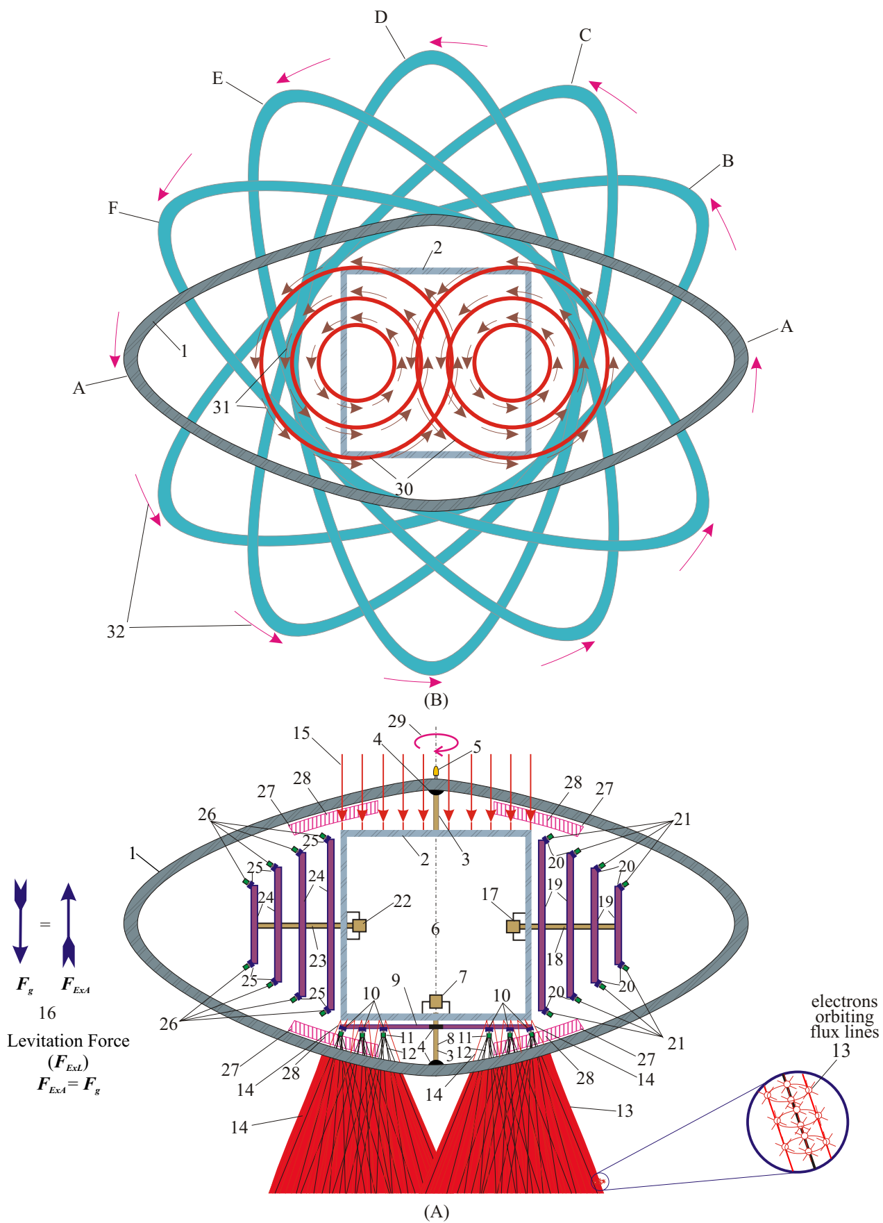
Fig.9. The spinning mechanism of Ski-Kush ( S-Kush ). In (A) leakage field from ExMF diverted by the ferromagnetic material 1. In (B), circles of rotating ExMF are shown by arrows, leakages fields 15 interacted with solenoid's magnetic fields 28 resulted in motor action, thus spinning the external diamagnetic body 1 along the vertical axis 3 in (A), direction of rotation is shown by arrows 29 in (B). As the external body 1 rotates from states A to B, C, D, E, F back to A in continual spinning motion, the internal body 2 with its occupants and control instruments are kept stable like gyroscope.
