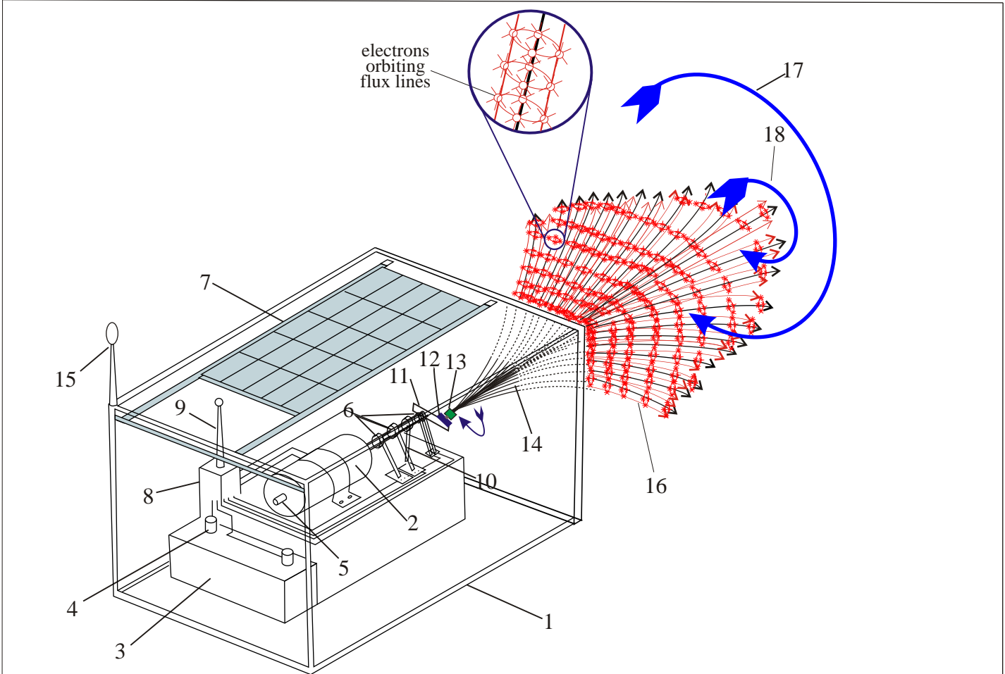
Fig.1. Machine to capture and energized charged particles (electrons and protons) by producing external magnetic field ( ExMF ).
