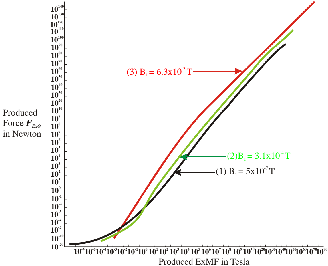
Graph 1. The relationship between produced External Magnetic Field ( ExMF ) and the resulted ExMF operational force ( F_{Ext} ), for three (3) given Rotating Low Magnetic Field ( RLMF ) or ( B_1 ).
